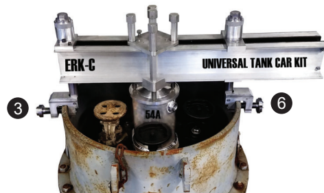
CHLORINE TANK-CAR APPLICATION
